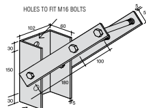
SBK37 ■ INCLUDES 2 M16X140 BOLTS (B155)
