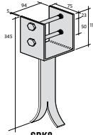
SBK8 ■ INCLUDES 2 M12X120 HDG BOLTS (B138)
